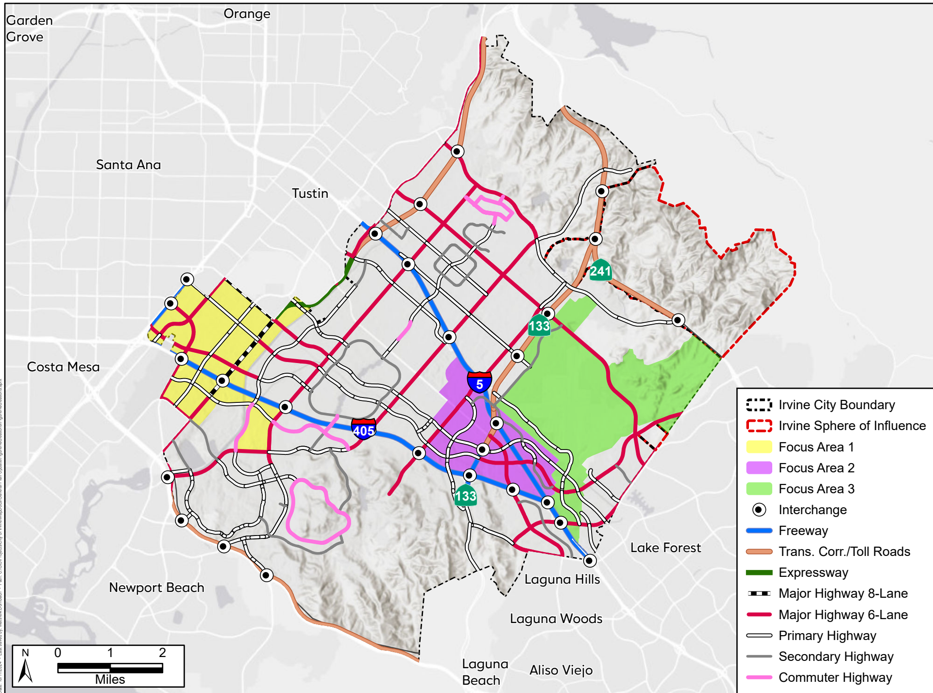
Figure 1. Master Plan of Arterial Highways
